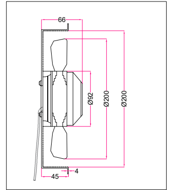
FAN WITH FLAT / BASKET GRILL
