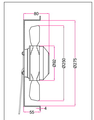
FAN WITH FLAT/BASKET GRILL
